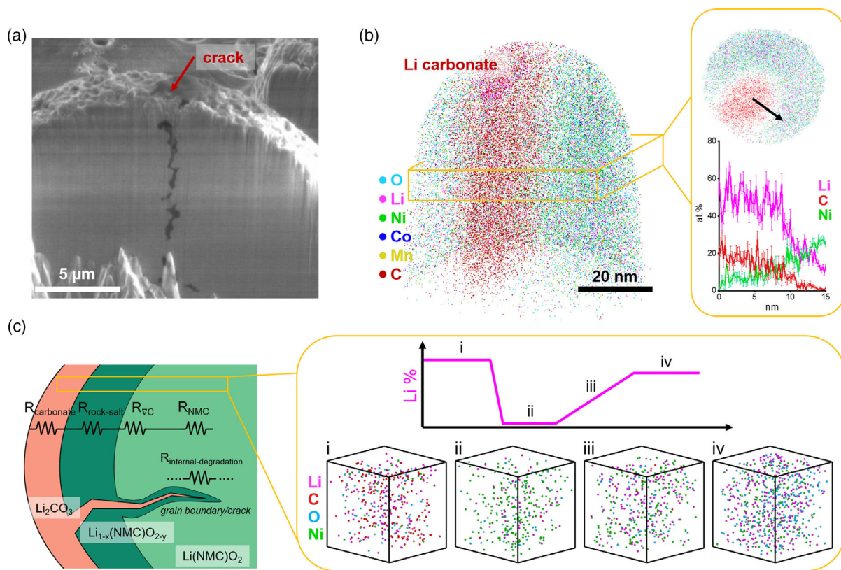
Figure 4. a) Cross-sectioned air-stored NMC particle. b) APT result of the NMC with \text{Li}_2\text{CO}_3 . The specimen was prepared by the non-cryo protocol. The orange box shows (top) the 5 nm-thin-sliced tomogram along the APT measurement direction and (bottom) atomic compositional profile at the interface marked by the black arrow in the tomogram. c) A schematic illustration of NMC 811 material after air oxidation with an arbitrary Li concentration profile along the surface. Note that the insets show the extracted cuboidal volume ( 3 \times 3 \times 3 \text{ nm}^3 ) of each different layer: \text{Li}_2\text{CO}_3 , Ni-rich oxides, diffusion profile, and NMC particles. Pink, red, blue, and green spheres represent the reconstructed Li, C, O, and Ni atoms. Additionally, Figure S11, Supporting Information, shows many air-susceptible sites for NMC particles: grain boundaries, cracks, triple junction, surface, etc.
