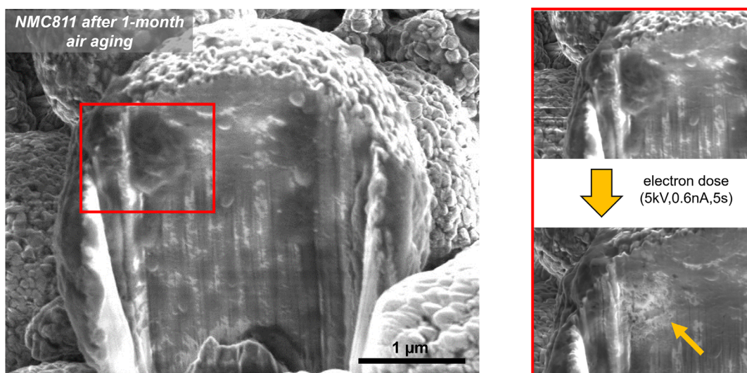
Figure 2. Electron beam-induced decomposition of \text{Li}_2\text{CO}_3 layers on air-aged NMC particle. Yellow arrow remarks the deformation induced by electron beams. Additional information is shown in Figure S3, Supporting Information.
