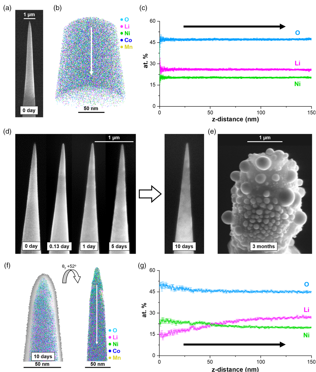
Figure 1. a) SEM image and b) 3D atom map of NMC811 APT specimen. c) Corresponding 1D atomic compositional profile along the measurement direction (white arrow in (b)). d) Ex situ oxidation experiment at different time span. e) NMC specimen after 3 month oxidation in ambient condition. f) APT specimen after 10 days oxidation and electron beam exposure for imaging. Inset image shows 3D atom map results with tilted at 52° in \gamma -axis. g) Corresponding 1D atomic compositional profile along the measurement direction (white arrow in (f)). Co and Mn elements are not shown.
