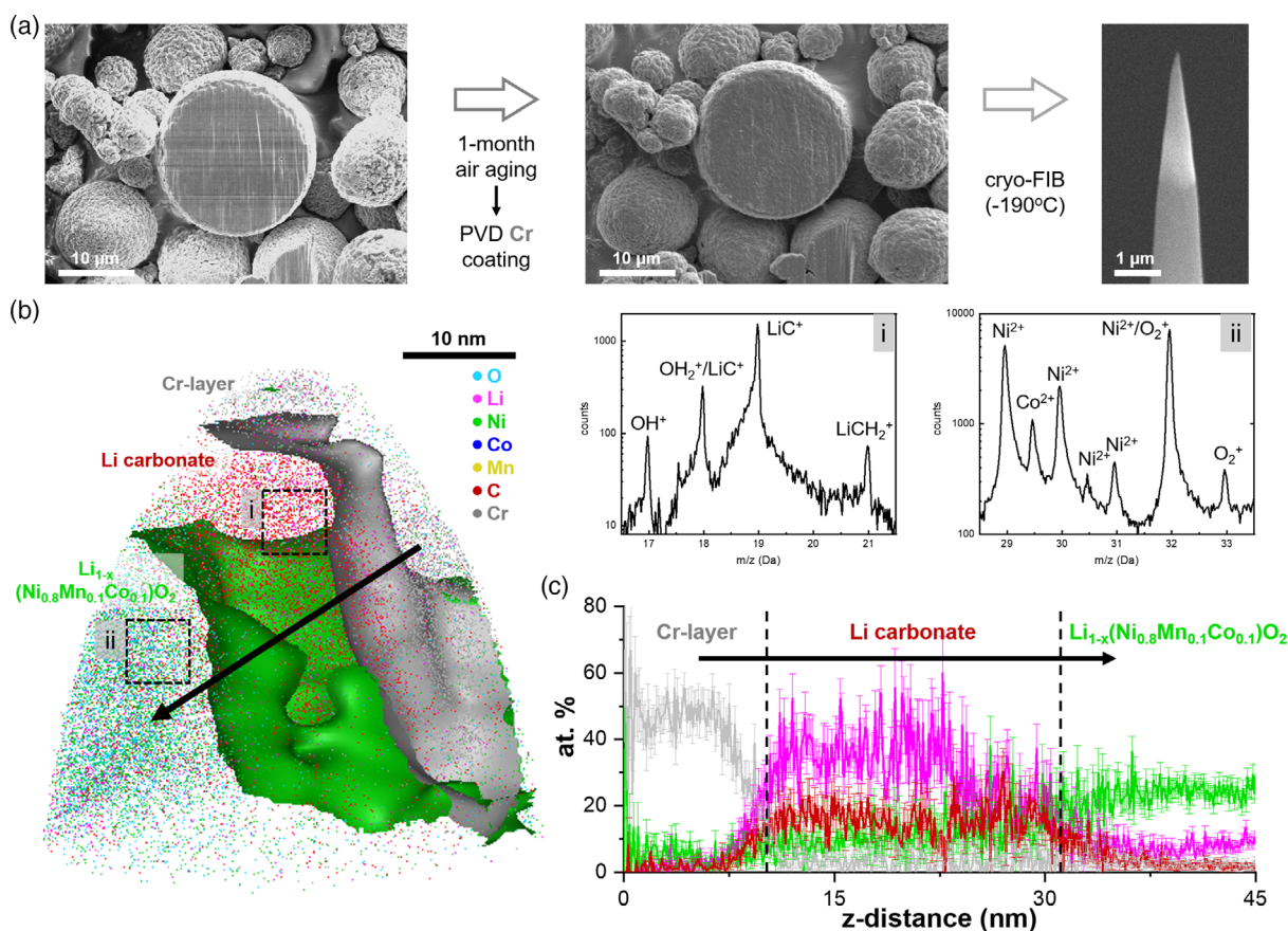
Figure 3. Atomic chemistry analysis of a month oxidized NMC particle. a) The APT specimen preparation of surface-sensitive material with PVD coating and cryogenic milling. No electron beam imaging was done before the PVD-Cr coating and 1 month ambient storage. b) 3D atom map of Cr-coated oxidized NMC surface. Inset i and ii display extracted local mass spectra of interest regions in (b). In the extracted mass spectrum of the impurity layer, it indeed shows the peak of Li-C molecular ions that we can conclude the presence of \text{Li}_2\text{CO}_3 . c) 1D compositional profile of elements across the oxidized NMC surface (cylindrical region of interest of \Phi 5 \times 50 \text{ nm}^3 ). Co, Mn, and O elements are not plotted. The details of the mass spectrum analysis are presented in Figure S9, Supporting Information.
