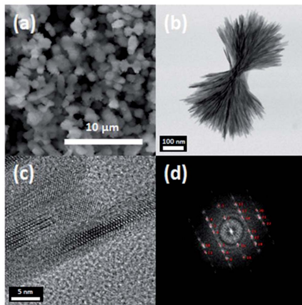
Fig. 3 (a) SEM image of nano urchin-shaped LiFePO 4 nanoparticles (NU-LFP NPs), (b) and (c) HRTEM images of the NU-LFP NPs, and (d) fast Fourier transform images of NU-LFP NPs.
