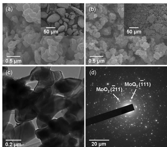
Figure 1. The FE-SEM images of the (a) raw \text{MoO}_2 and (b) ballmilled \text{MoO}_2 . The HR-TEM image of the (c) raw \text{MoO}_2 and (d) SAED pattern.
